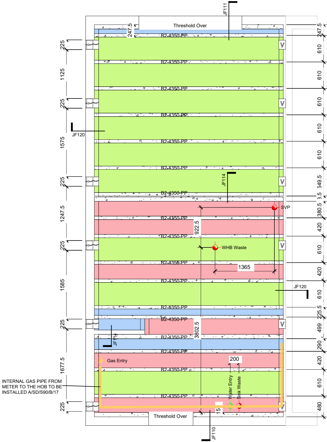
1 Beam Layout 1-50 1 : 50
